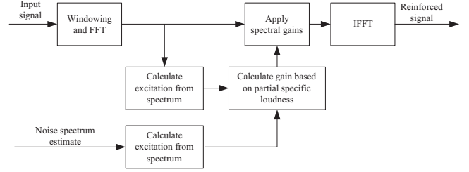
Fig. 3. Block diagram of proposed speech reinforcement system
