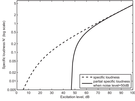
Fig. 2. Moore's models for specific loudness and the partial specific loudness of the 1 kHz tone when the noise excitation level is 50 dB as functions of the signal excitation level (Eqs. (1) and (3)).
