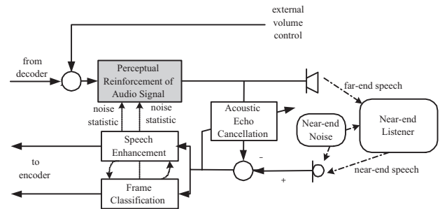
Fig. 1. Block diagram of a communication system in adverse environment.
