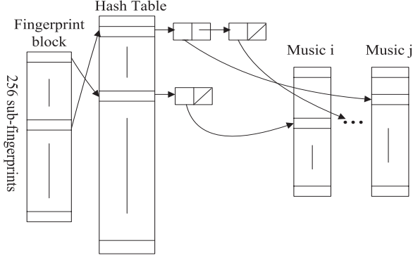
Fig. 2. Fingerprint matching stage of PRH
