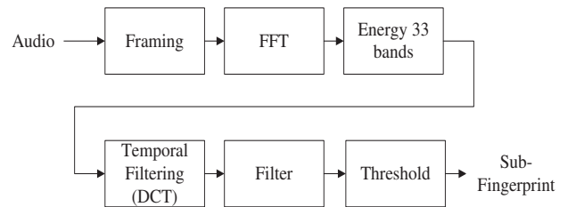
Fig. 3. Fingerprint extraction stage of MLH
