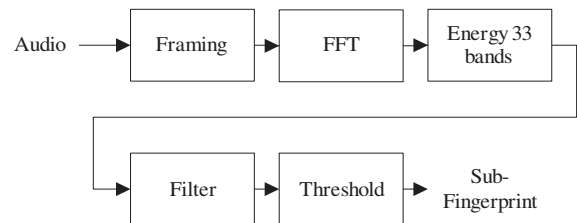
Fig. 1. Fingerprint extraction stage of PRH [6]
