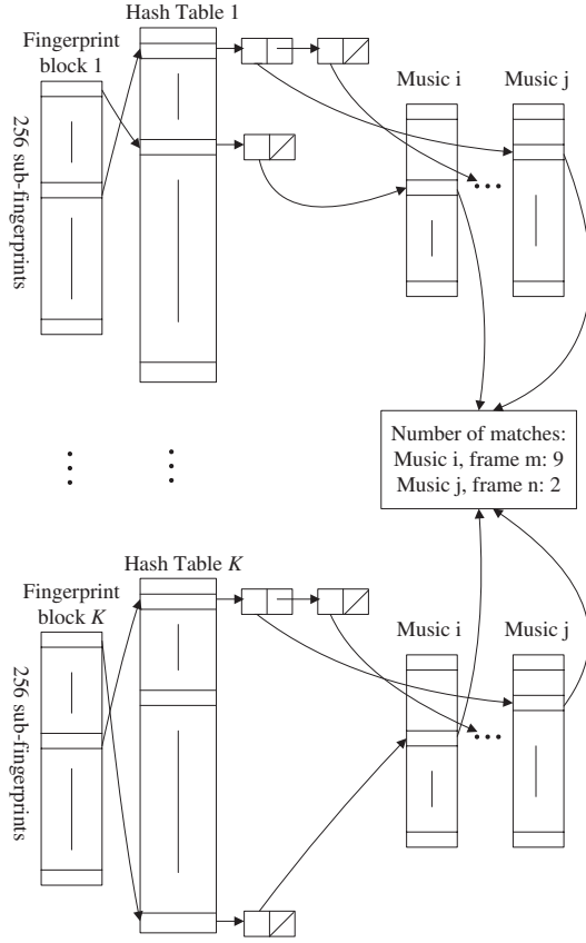
Fig. 4. Fingerprint matching stage of MLH
